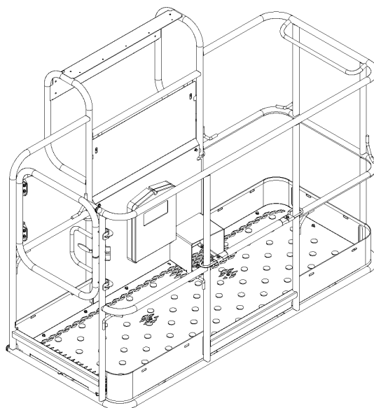
(1) Side Swing Gate Platform
